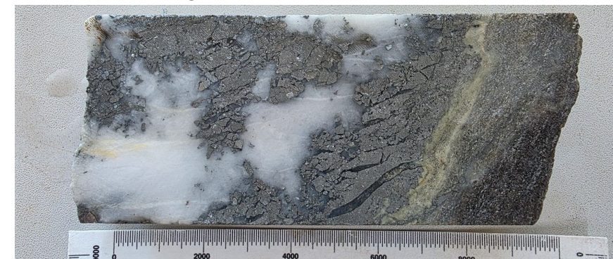
TBS_018, 0.52m @ 14.1 g/t Au, 16.1 g/t Ag 2
