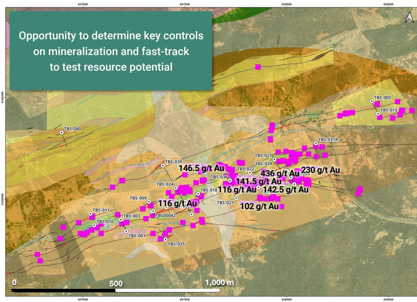
Main zone geology map showing drilling and rock chips (>20 g/t Au) 1
